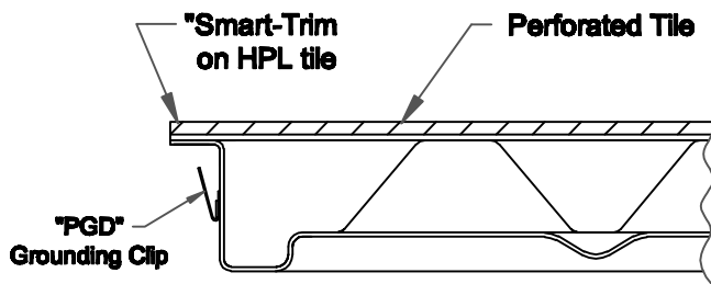
PARTIAL SIDE VIEW
