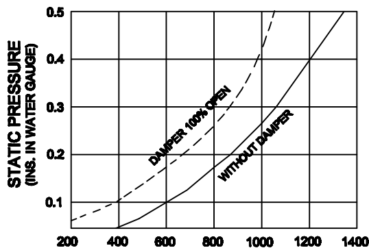
VOLUME OF AIR FLOW (C.F.M.)
