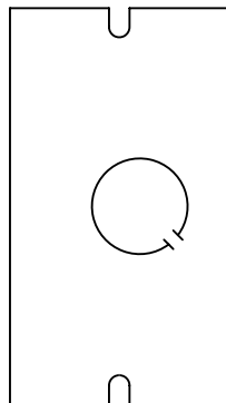
DP001 Cable Conn. Plate With 1/2" Knockout
