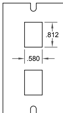
DP007 For (2) Modular Jack Couplers
