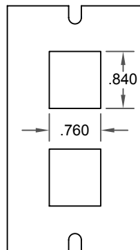
DP011 For (2) Modular Jack Couplers
