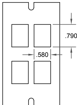
DP010 For (4) Tyco SL-110 Jacks
