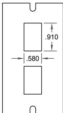
DP006 For (2) Modular Jack Couplers
