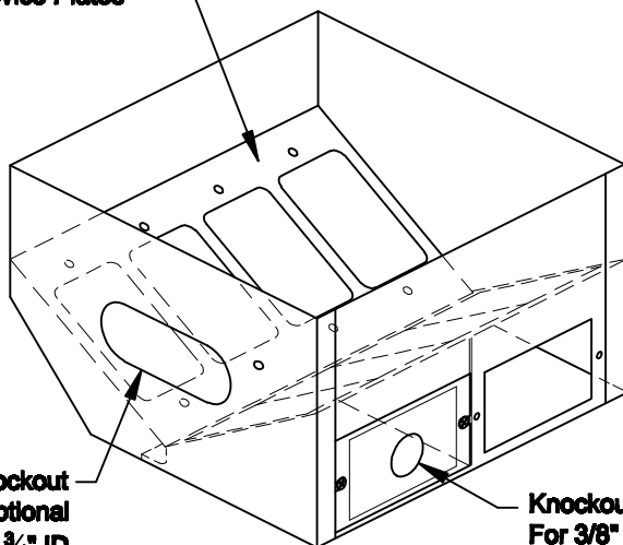
REAR VIEW (Shown With Lid Removed)
